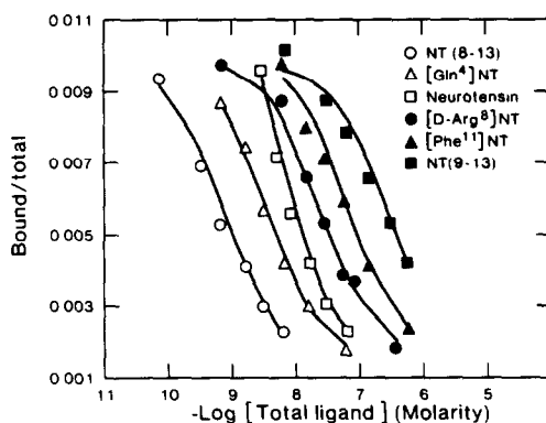
Fig. 5. Effect of concentration on inhibition of [ ^3\text{H} ]neurotensin binding to clone N1E-115 by neurotensin and some of its analogs and fragments. The data presented are representative of the competition curves obtained when increasing concentrations of neurotensin and its analogs and fragments were assessed for their ability to compete with [ ^3\text{H} ]neurotensin for binding to intact cells employing the modified assay procedure described under Materials and Methods. Cells used for these assays were cultured in DMEM with 10% fetal bovine serum. Each point is the average of duplicates, and the inhibition curves were generated with the LIGAND computer program [16]. Complete data on all the neurotensin peptides and their apparent equilibrium dissociation constants and Hill coefficients are presented in Table 2.
