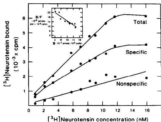
Fig. 1. [ ^3\text{H} ]Neurotensin binding to clone N1E-115 as a function of radioligand concentration. The binding of increasing concentrations of [ ^3\text{H} ]neurotensin to intact N1E-115 cells was performed at 0^\circ as described under Materials and Methods with 0.4 \times 10^6 cells/assay tube (cells in stationary phase of growth; passage number 9; 12 days after subculture in DMEM with 10% newborn calf serum). Specific binding was obtained by subtracting the average of duplicates for nonspecific binding at a given radiolabel concentration (measured in the presence of 1 \mu\text{M} unlabeled neurotensin) from the average of duplicates for total binding. Each point represents the average of duplicates, and the data presented are from one of four similar neurotensin binding assays. Inset represents a Scatchard plot of the given specific binding data fitted with the least squares method of linear regression analysis.
